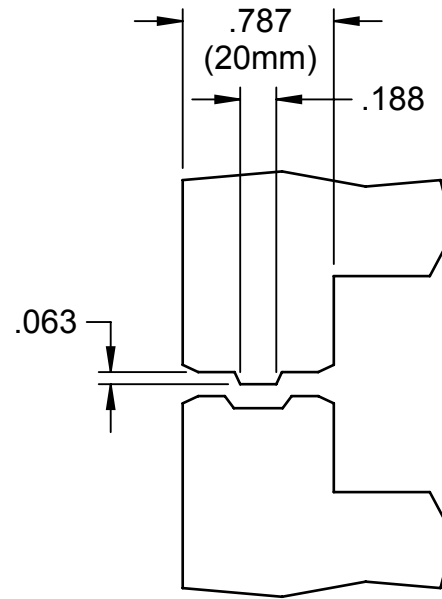
M593/F575 FORMS
