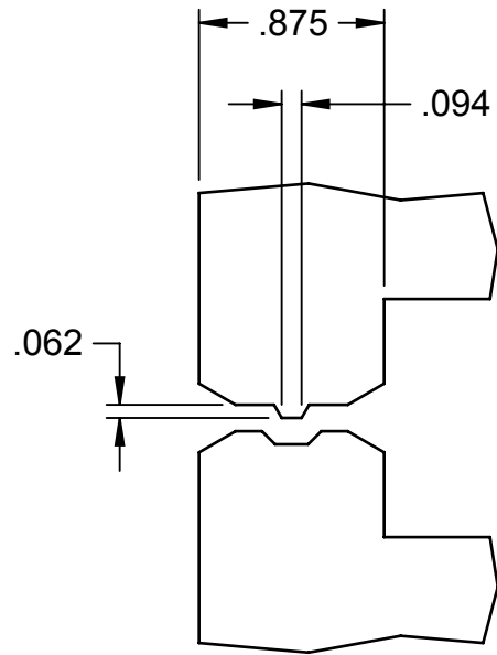
M3/F4 FORMS
