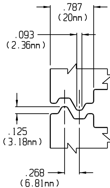
"OFFSET" M707/F648 FORMS
