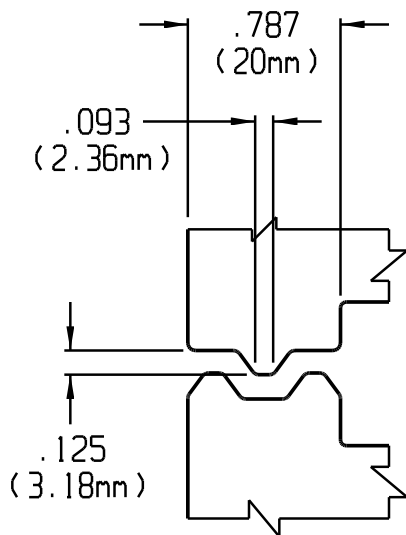
"3-POINT" M684/F632 FORMS
