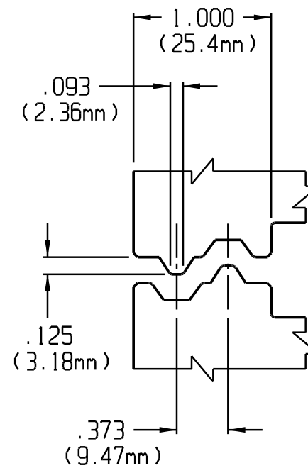
"FIXED CENTER OFFSET" M743/F673 FORMS
